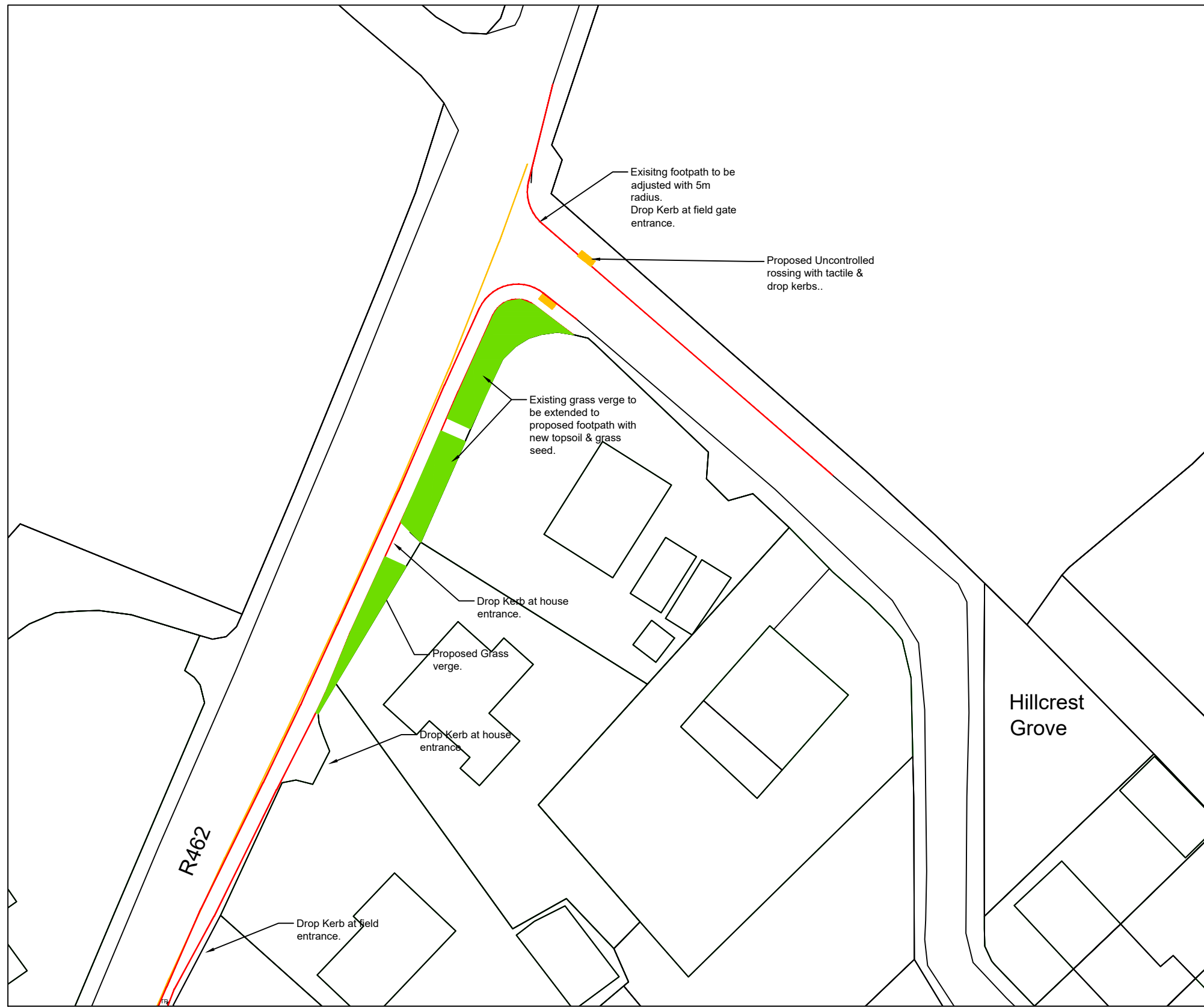
SITE LOCATION PLAN Extract from O.S. 4384-C Scale: 1/500
